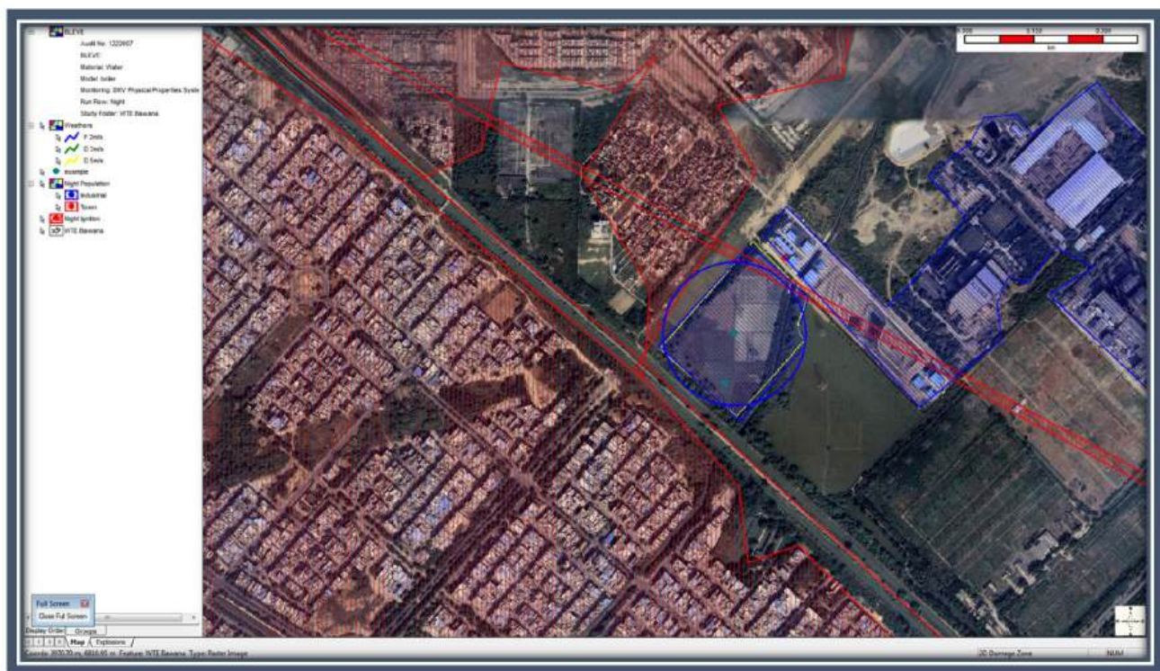
Fig. 7.4 Damage Contour for BLEVE Scenario at WtE Bawana for Boiler
