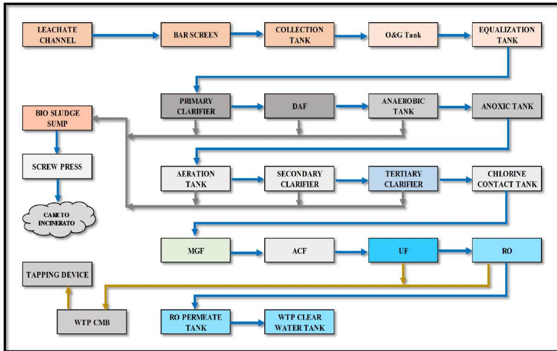
Figure 2.7: LTP Process Flow Diagram
