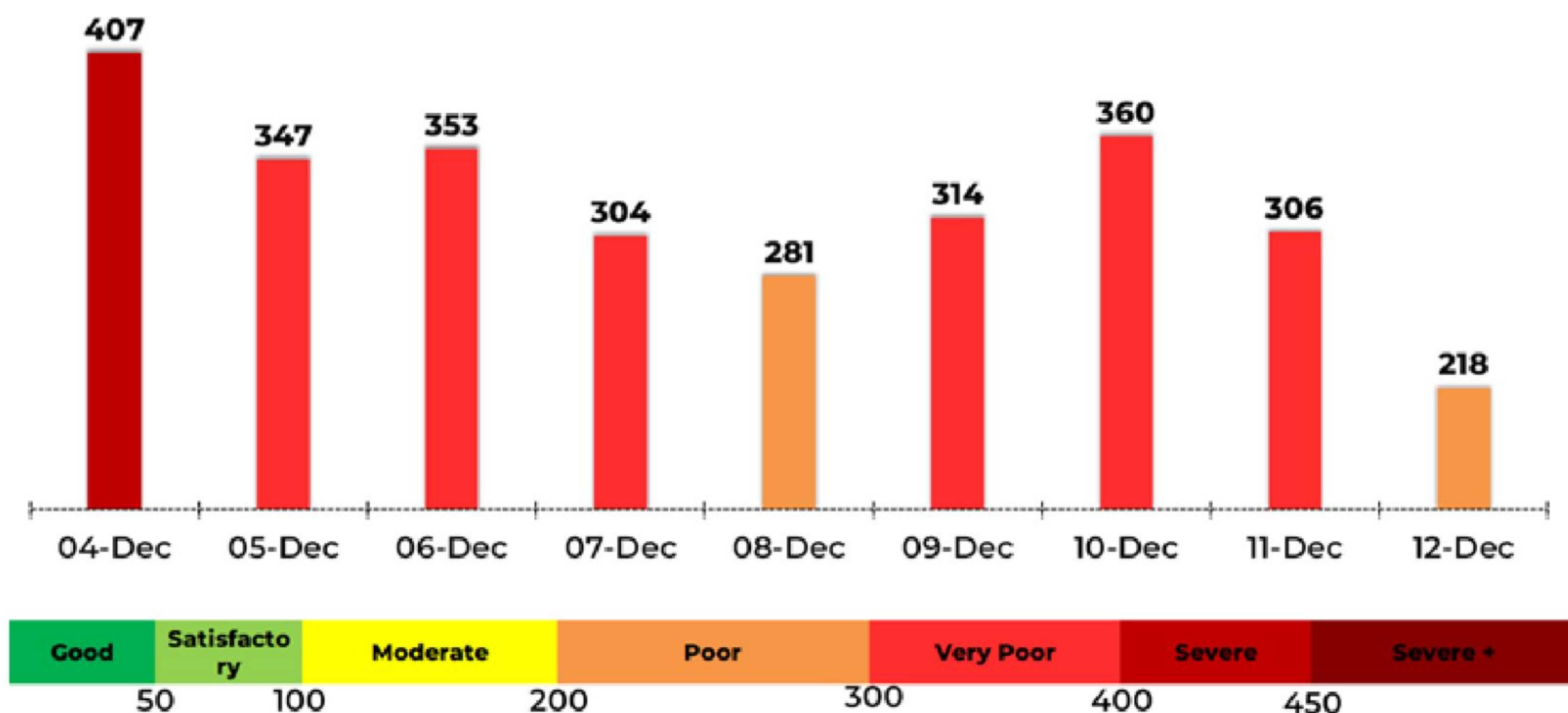
Air Quality during last 7 days
